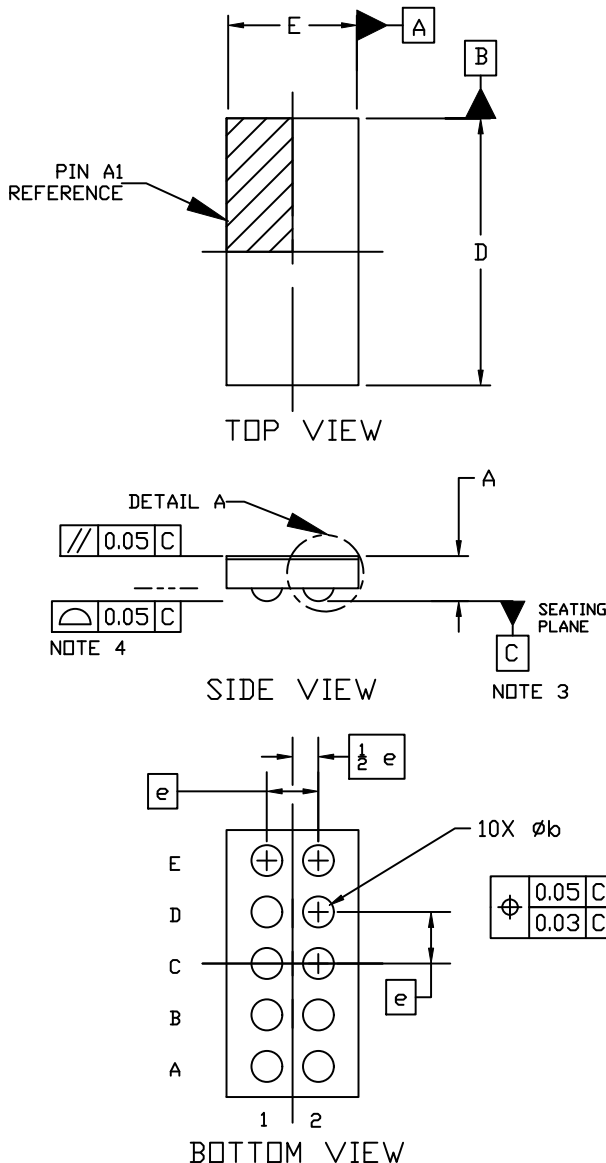
WLCSP10, 2.075x1.025x0.35 CASE 567ZC ISSUE O
