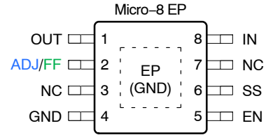
Figure 4. Pin Assignments
