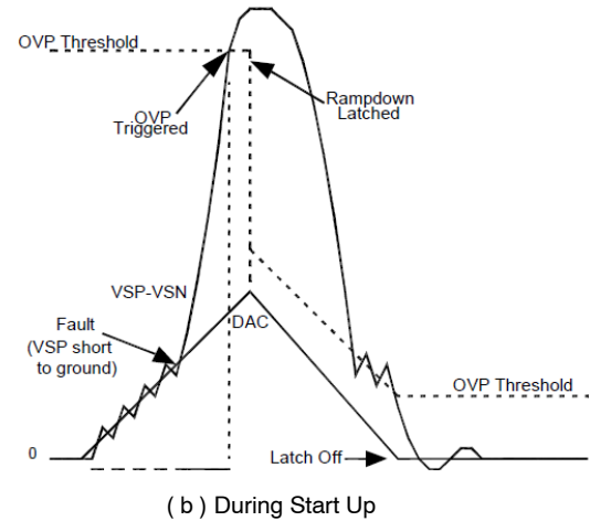
Figure 17. Function of Latch-Off Over Voltage Protection
