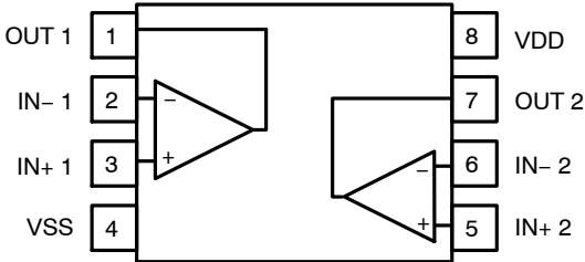
Figure 1. Pin Connections
