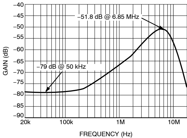
Figure 7. SD Channel-to-Channel Crosstalk
