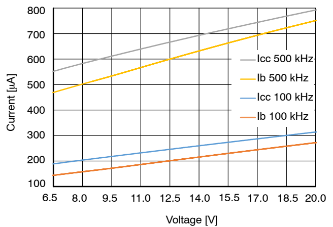
Figure 35. Current Consumption vs. Voltage. Load = 0 nF
