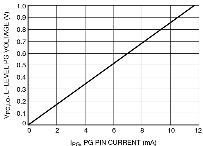
Figure 16. L-level PG Voltage vs. Current
