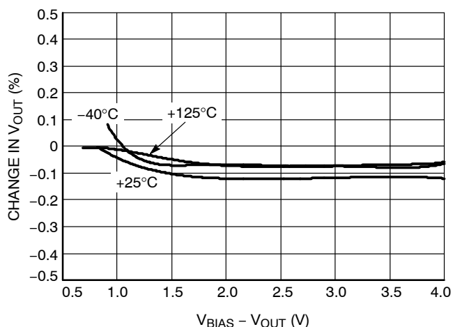
Figure 6. V_{BIAS} Line Regulation
