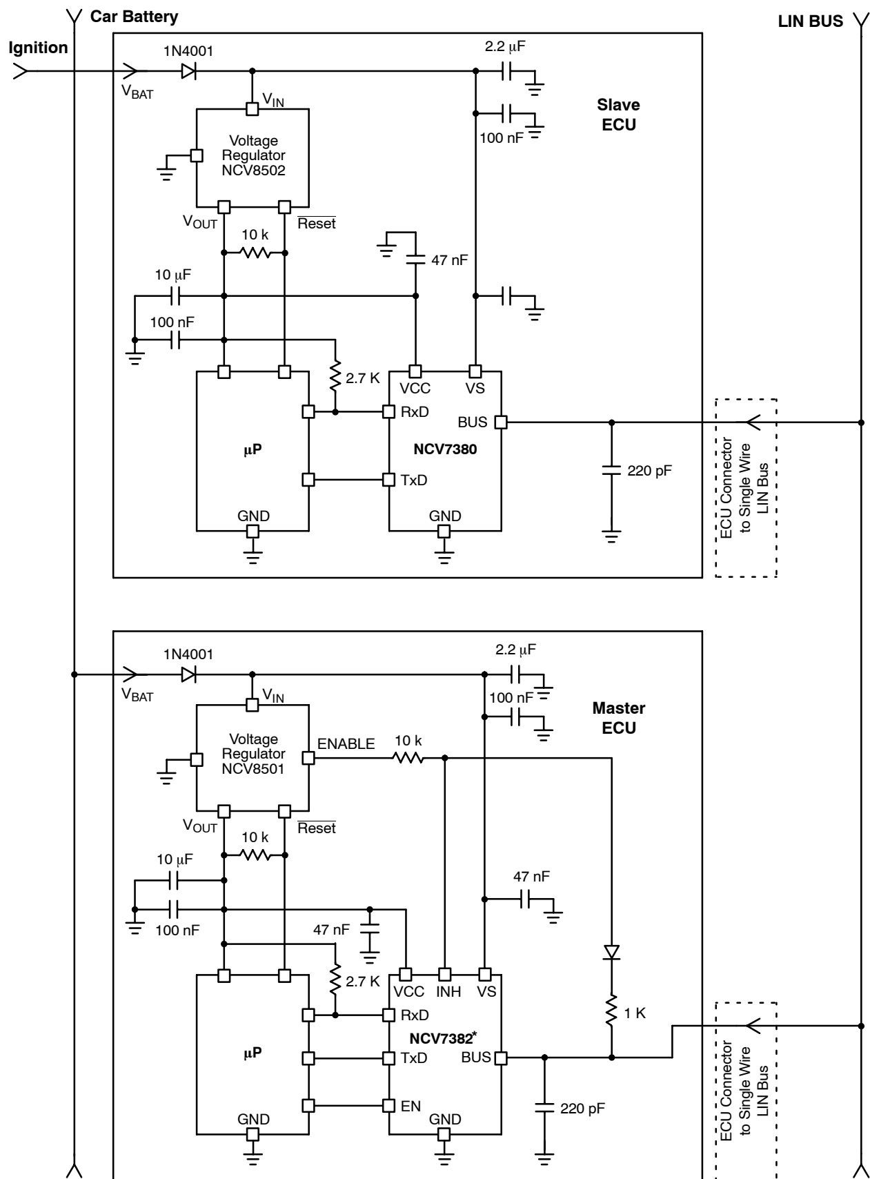
Figure 9. Application Circuitry
