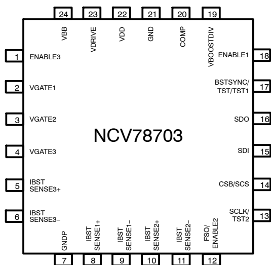
Figure 3. Pin Connections – QFNW24 5x5 and QFNW24 4x4
