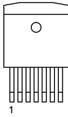
D²PAK-7
