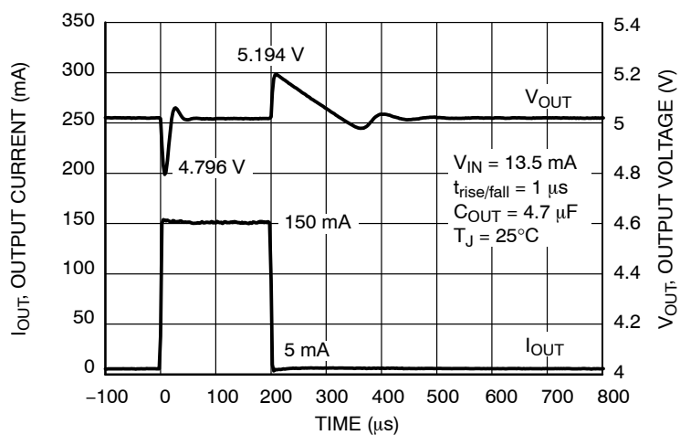
Figure 24. Load Transients
