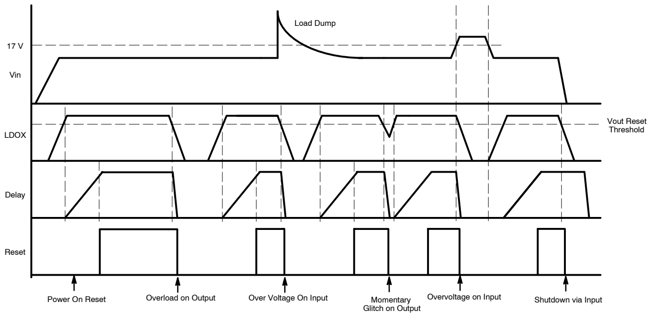
Figure 4. NCV8613 Reset Timing Diagram
