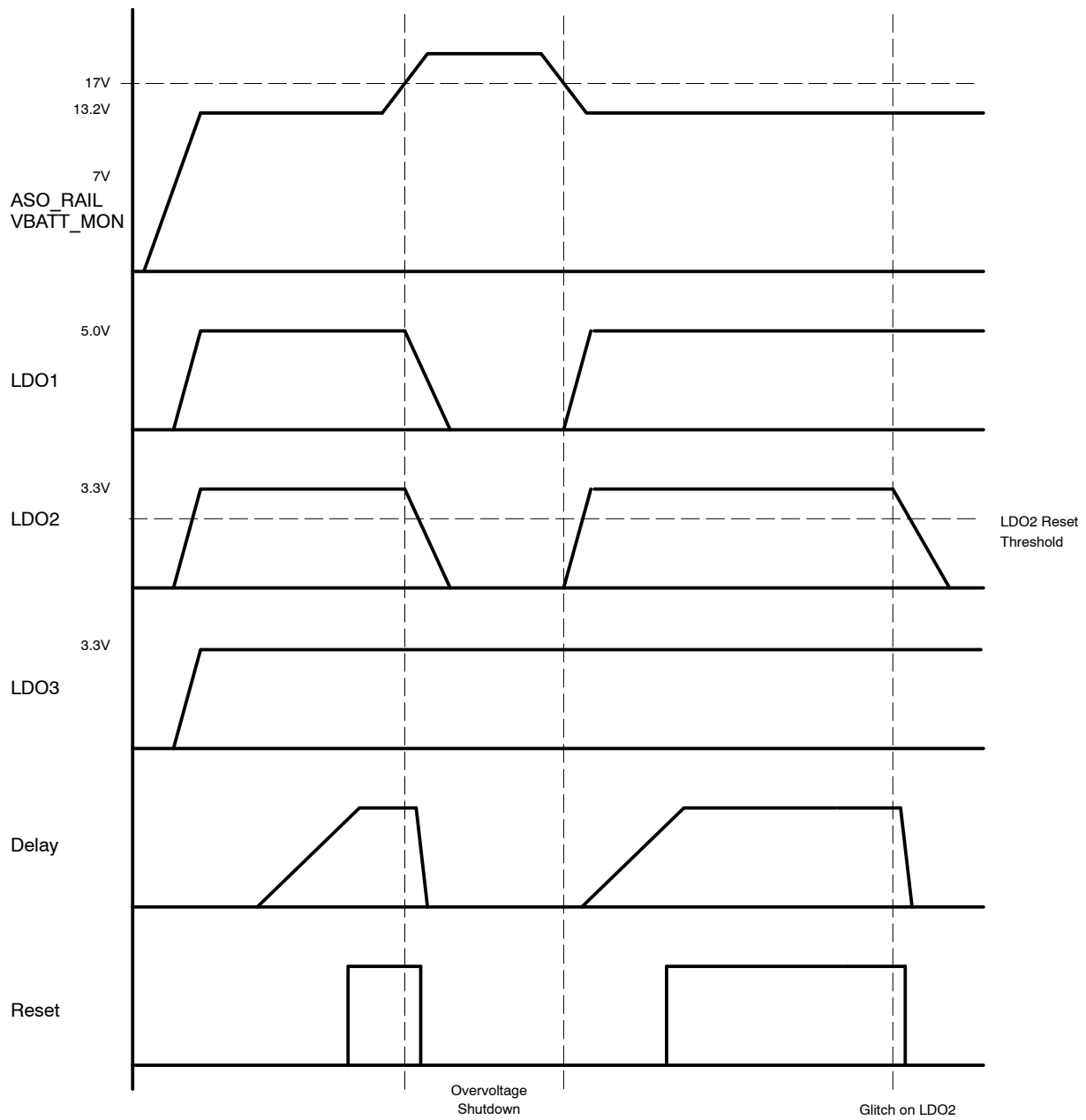
Figure 9. NCV8613 Regulator Output Timing Diagram– VIN_S3 Tied to ASO_RAIL
