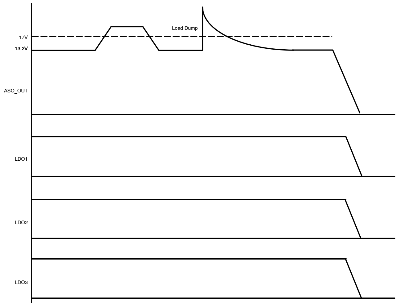
Figure 10. NCV8613 Regulator Output Timing Diagram– VBATT_MON Grounded
