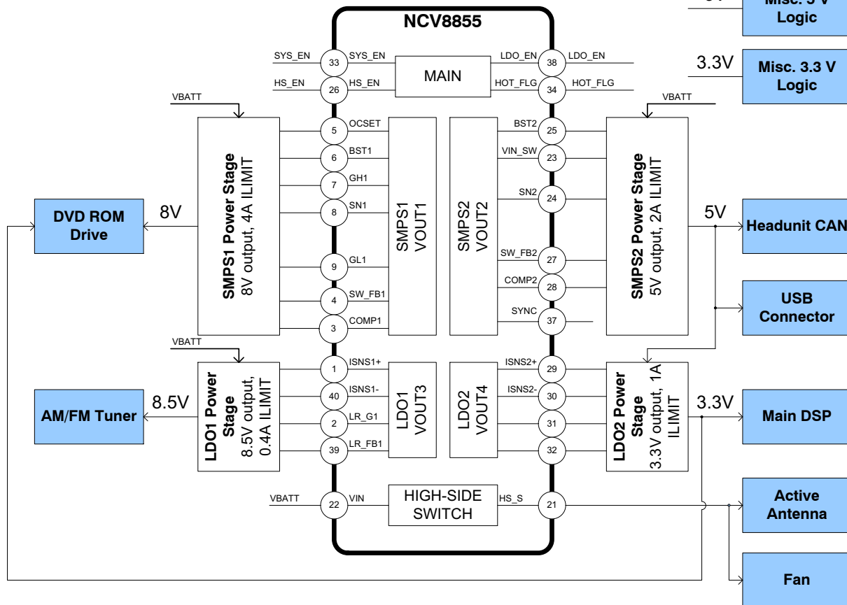
Figure 2. Automotive Radio System Block Diagram Example NCV8613 with NCV8855
