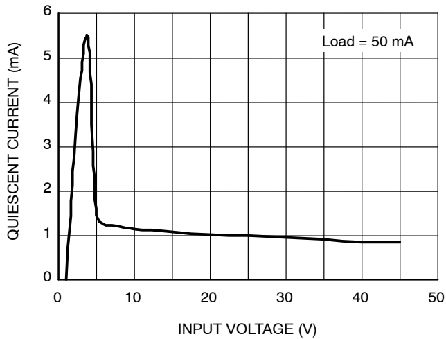
Figure 8. NCV8675 Quiescent Current vs. Input Voltage (5 V Version)
