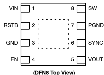
(DFN8 Top View)
