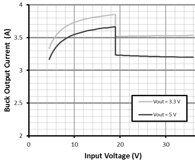
Figure 29. NCV891330 Load Current Capability with a 2.2 \mu\text{H} Inductor
