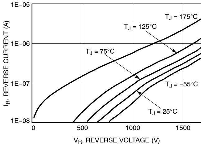
Figure 2. Reverse Characteristics
