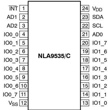
Figure 3. TSSOP24
