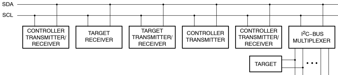
Figure 14. System Configuration
