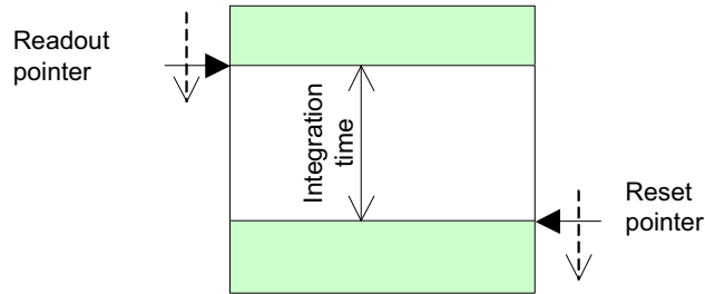
Figure 12. Electronic Shutter
