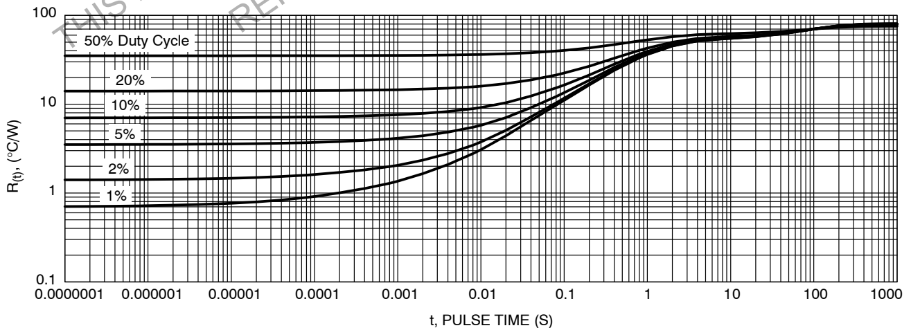
Figure 10. Transient Thermal Response, Junction-to-Ambient, for NRVTSF5100E
