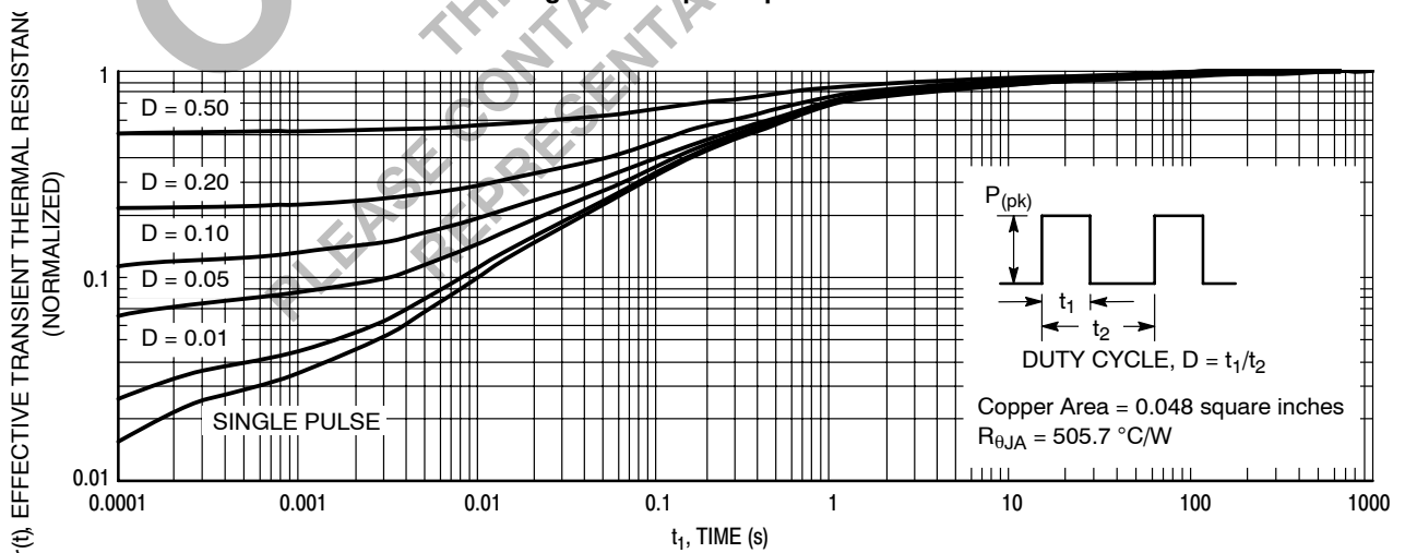
Figure 10. Normalized Thermal Response
