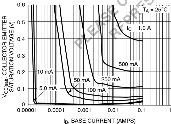
Figure 5. V_{CE(sat)} Collector Emitter Saturation Voltage vs. Base Current
