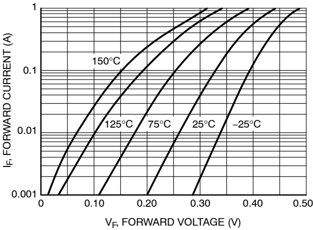
Figure 1. Forward Voltage
