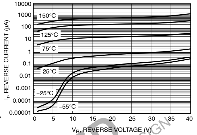
Figure 6. Leakage Current
