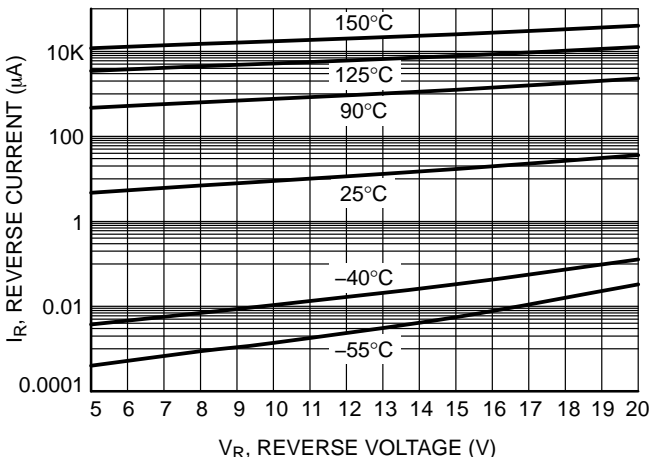
Figure 6. Leakage Current
