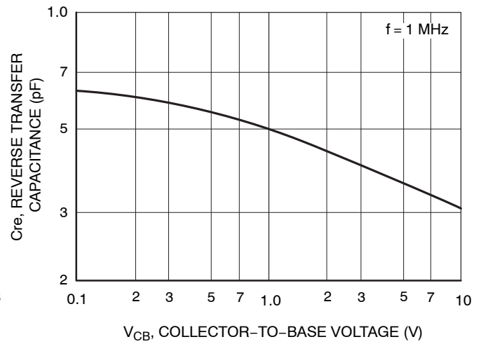
Figure 4. C_{re} - V_{CB}
