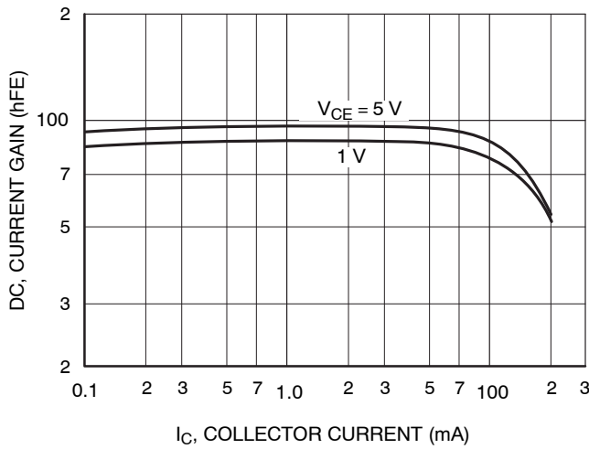
Figure 3. h_{FE} - I_C
