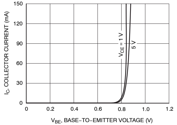
Figure 2. I_C - V_{BE}
