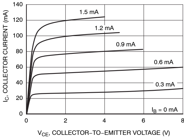
Figure 1. I_C - V_{CE}
