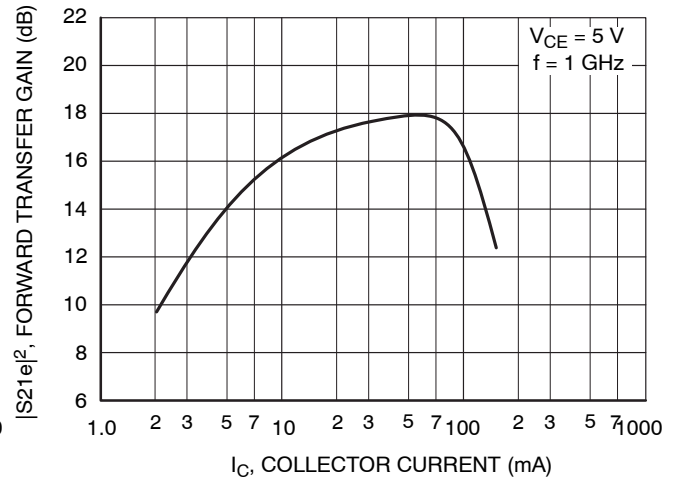
Figure 6. |S_{21e}|^2 - I_C
