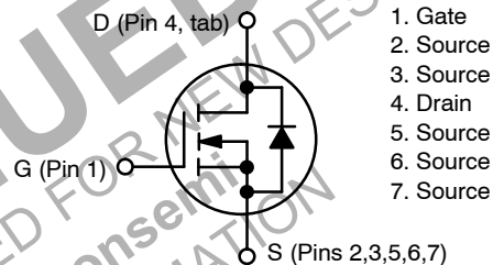
N-CHANNEL MOSFET
