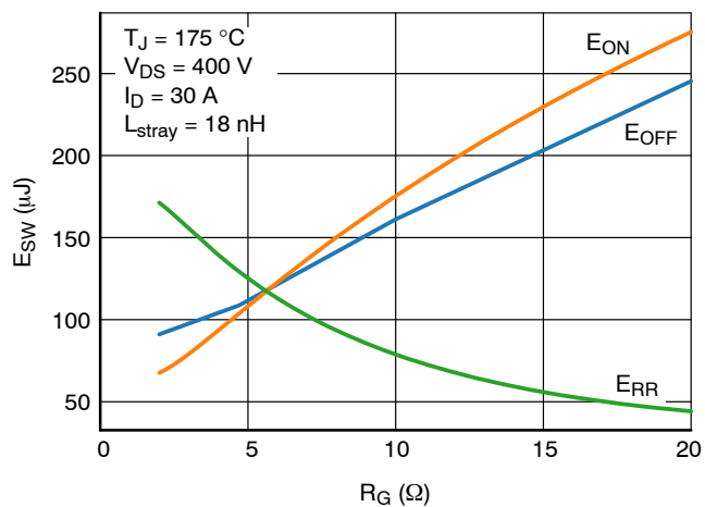
Figure 22. E_{SW} vs. R_G
