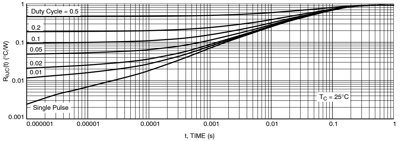
Figure 13. Thermal Impedance
