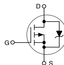
Single P-Channel
