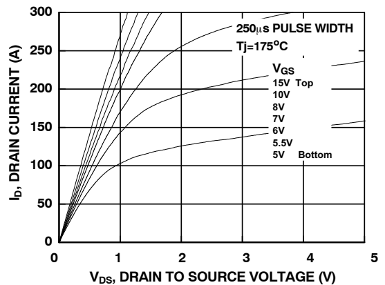
Figure 10. Saturation Characteristics
