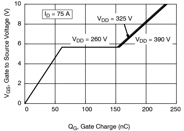
Figure 15. Gate Charge vs. Gate to Source Voltage
