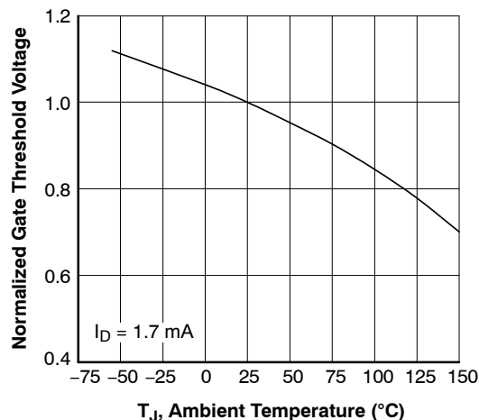
Figure 16. Normalized Gate Threshold Voltage vs. Temperature
