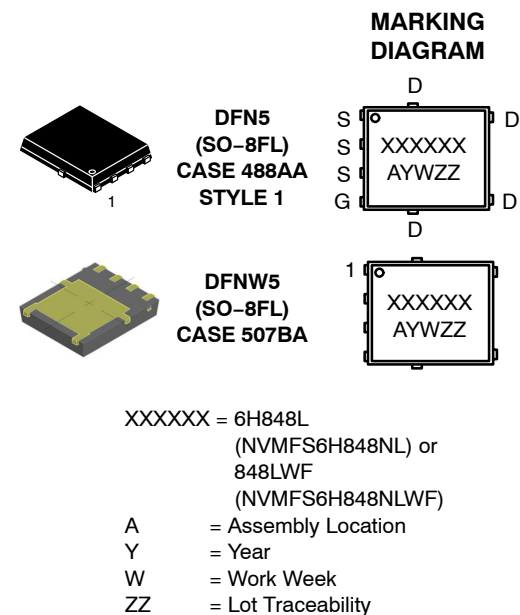
N-CHANNEL MOSFET
