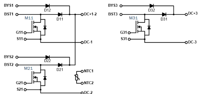
Figure 1. NXH80B120MNQ0SNG Schematic Diagram
