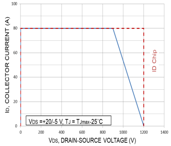
Figure 11. RBSOA
