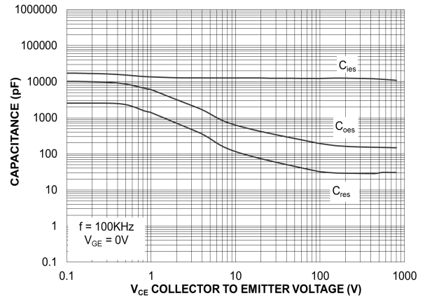
Figure 9. Capacitance
