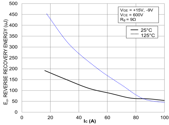
Figure 26. Typical Reverse Recovery Energy Loss vs. I C
