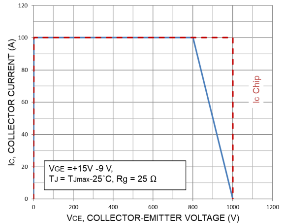
Figure 7. RBSOA
