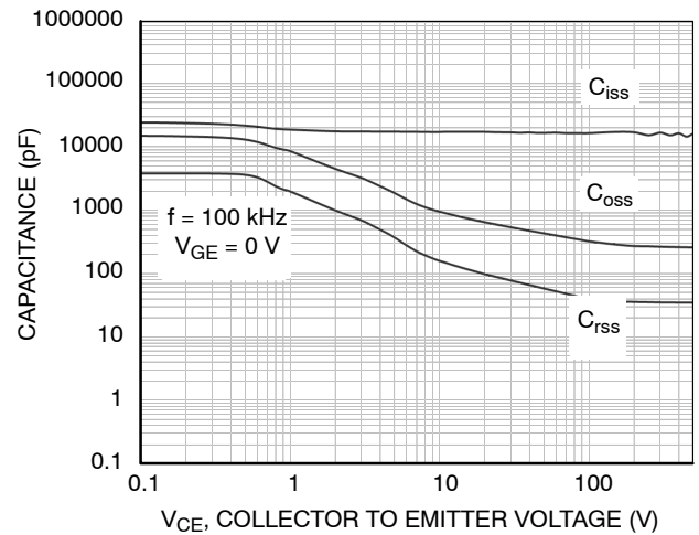
Figure 32. Capacitance
