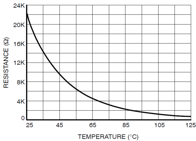
Figure 32. Thermistor Characteristics
