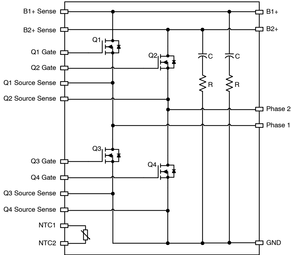
Figure 2. Schematic
