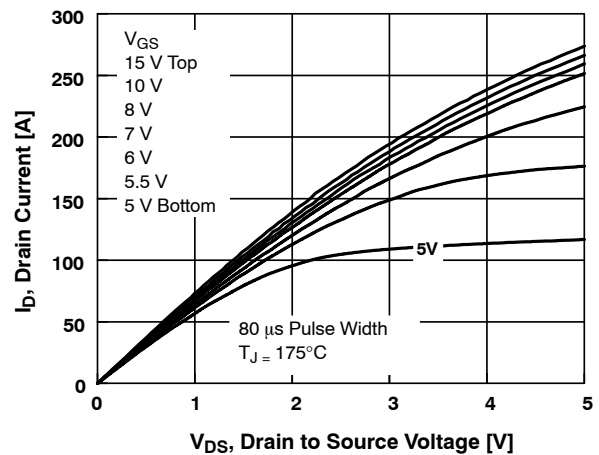
Figure 10. Saturation Characteristics
