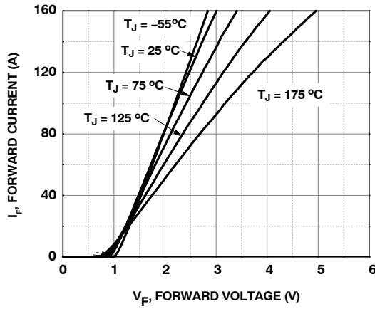
Figure 2. Forward Characteristics
