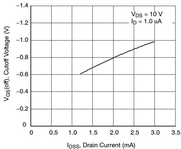
Figure 5. V_{GS(off)} - I_{DSS}
