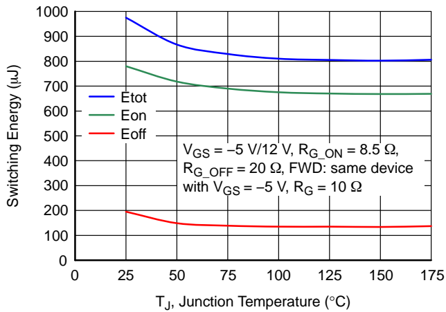
Figure 21. Clamped Inductive Switching Energy vs. Junction Temperature at V_{DS} = 800\text{ V} and I_D = 40\text{ A}
