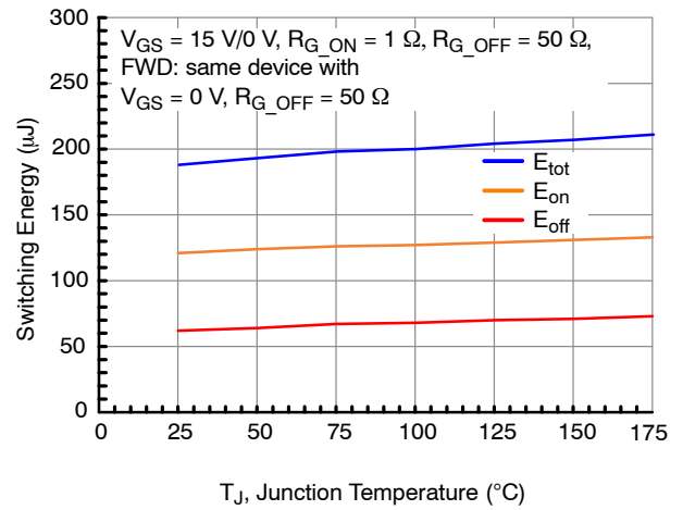
Figure 22. Clamped Inductive Switching Energy vs. Junction Temperature at V_{\text{DS}} = 400 \text{ V} and I_D = 25 \text{ A}
