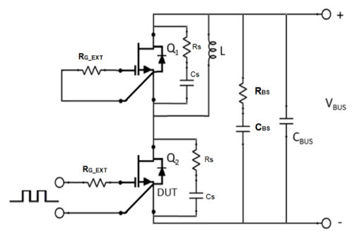
Figure 24. Schematic of the Half-Bridge Mode Switching Test Circuit with device RC Snubbers ( R_S = 10 \Omega , C_S = 68 \text{ pF} ) and a bus RC Snubber ( R_{\text{BS}} = 2.5 \Omega , C_{\text{BS}} = 100 \text{ nF} ).
