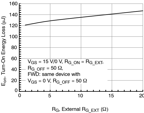
Figure 21. Clamped Inductive Switching Energies vs. R_{\text{G\_EXT}} at V_{\text{DS}} = 400 \text{ V} , I_D = 25 \text{ A} and T_J = 25^\circ\text{C}
