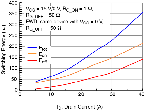
Figure 19. Clamped Inductive Switching Energy vs. Drain Current at V_{\text{DS}} = 400 \text{ V} and T_J = 25^\circ\text{C}
