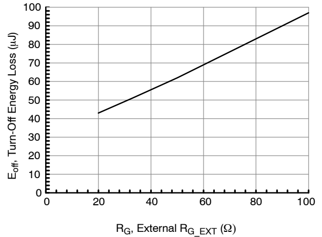
Figure 20. Clamped Inductive Switching Energies vs. R_{\text{G\_EXT}} at V_{\text{DS}} = 400 \text{ V} , I_D = 25 \text{ A} and T_J = 25^\circ\text{C}
