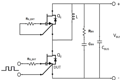
Figure 23. Schematic of the Half-Bridge Mode Switching Test Circuit. Note, a Bus RC Snubber ( R_{\text{BS}} = 2.5 \Omega , C_{\text{BS}} = 100 \text{ nF} ) is Used to Reduce the Power Loop High Frequency Oscillations.
