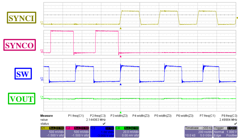
Figure 14. Starting synchronization at 2.5 MHz (from free-running)
