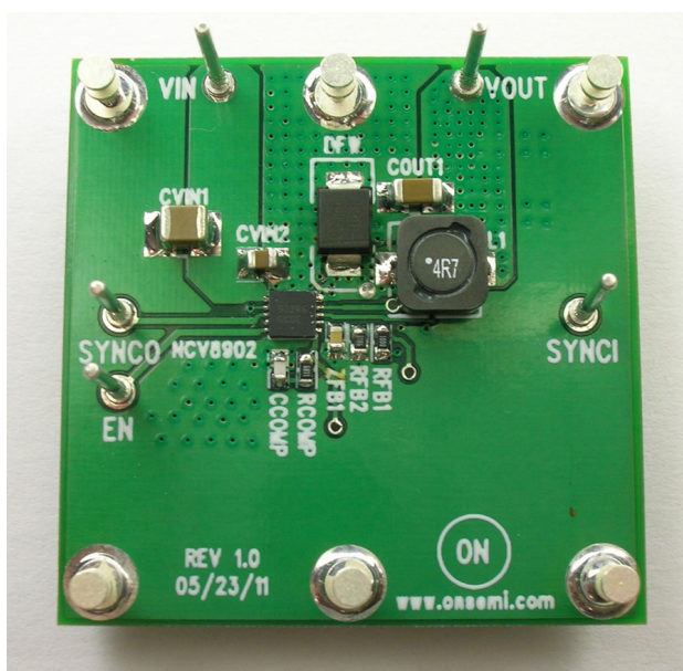
Figure 1. NCV890101GEVB Board Picture
