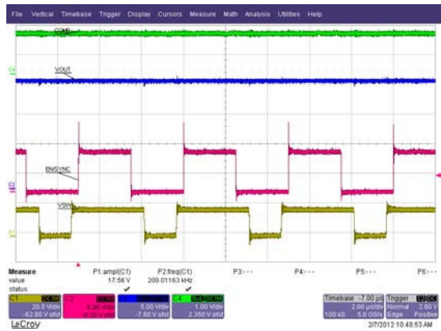
Figure 5. Synchronization
