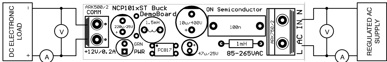
Figure 7. Test Setup
