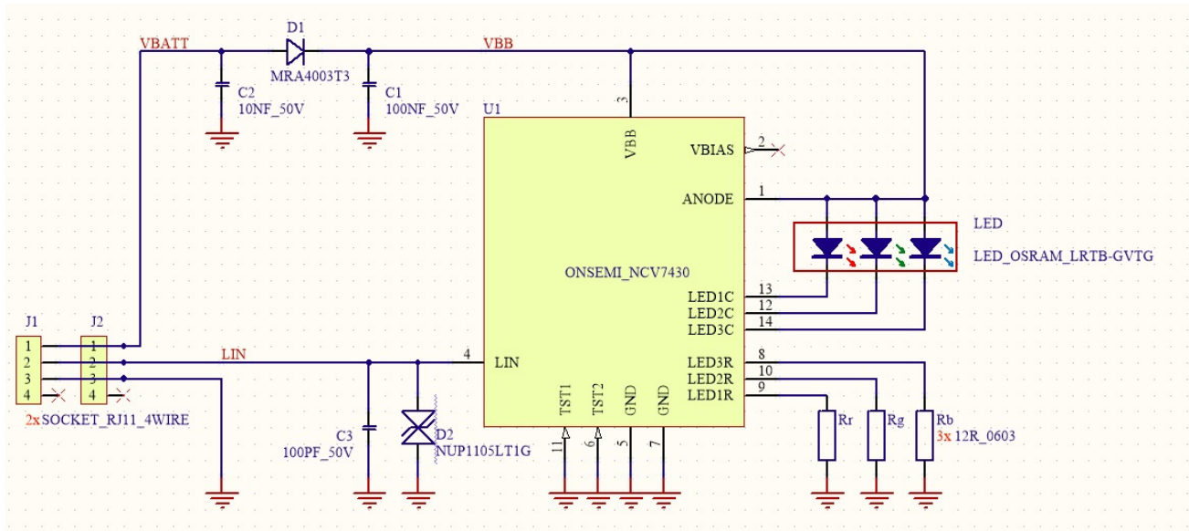
Figure 22. NCV7430 Schematic
