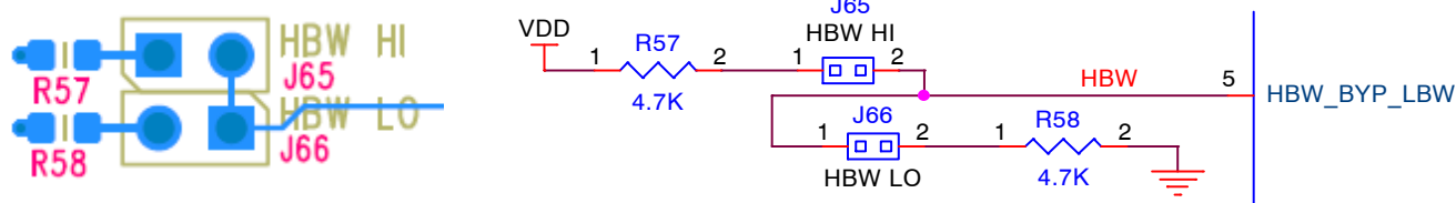
Figure 4. HBW_BYPASS_LBW# Schematic/PCB Configuration
