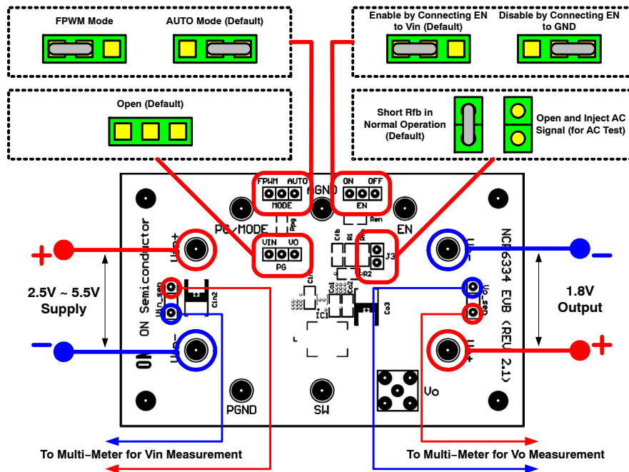
( b ) NCP6324C
