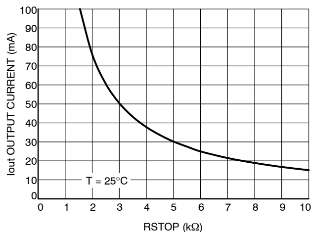
Figure 3. Iout vs. RSTOP
