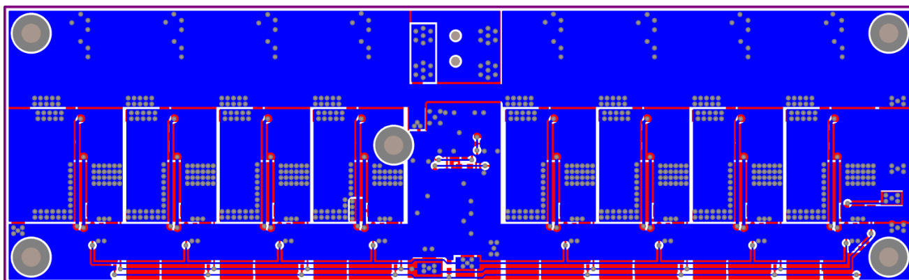
Figure 16. NCV7691 RCL/DRL EVB PCB Bottom Composite Drawing
